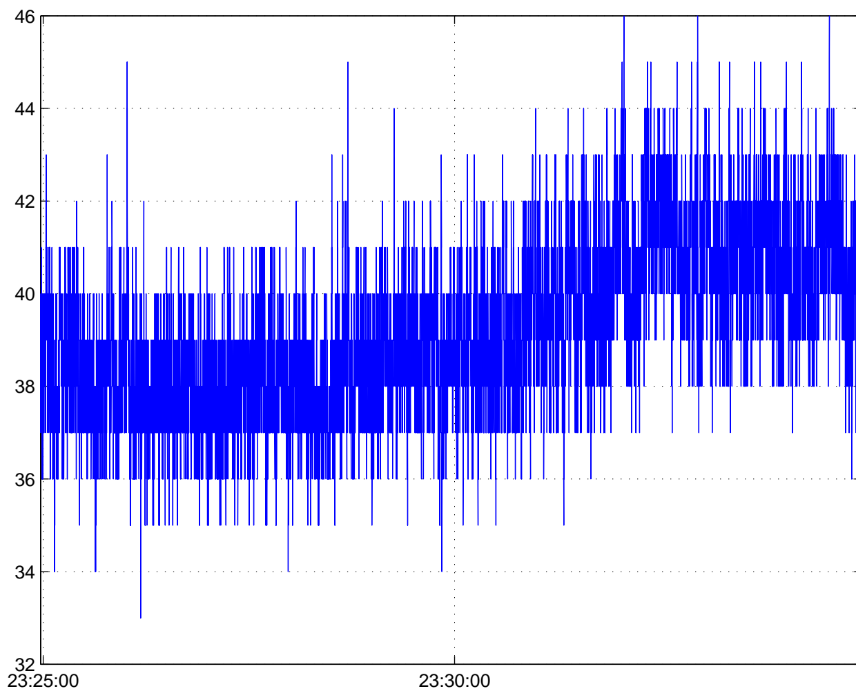
ATV tro FA, 2010-3-19 23:24:58 UT to 2010-3-19 23:34:57 UT
