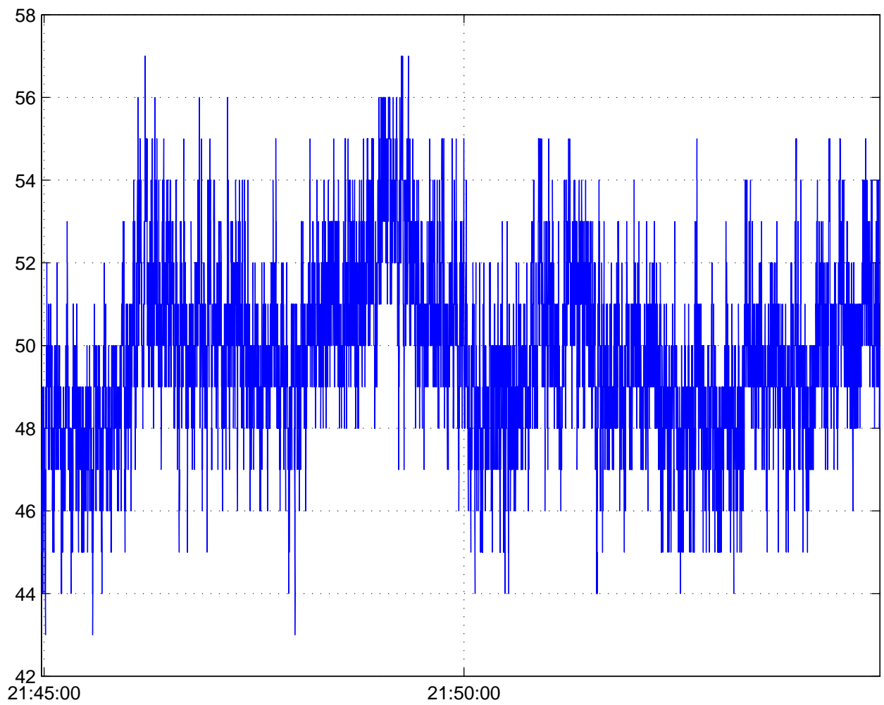
ATV tro FA, 2010-3-19 21:44:58 UT to 2010-3-19 21:54:57 UT
