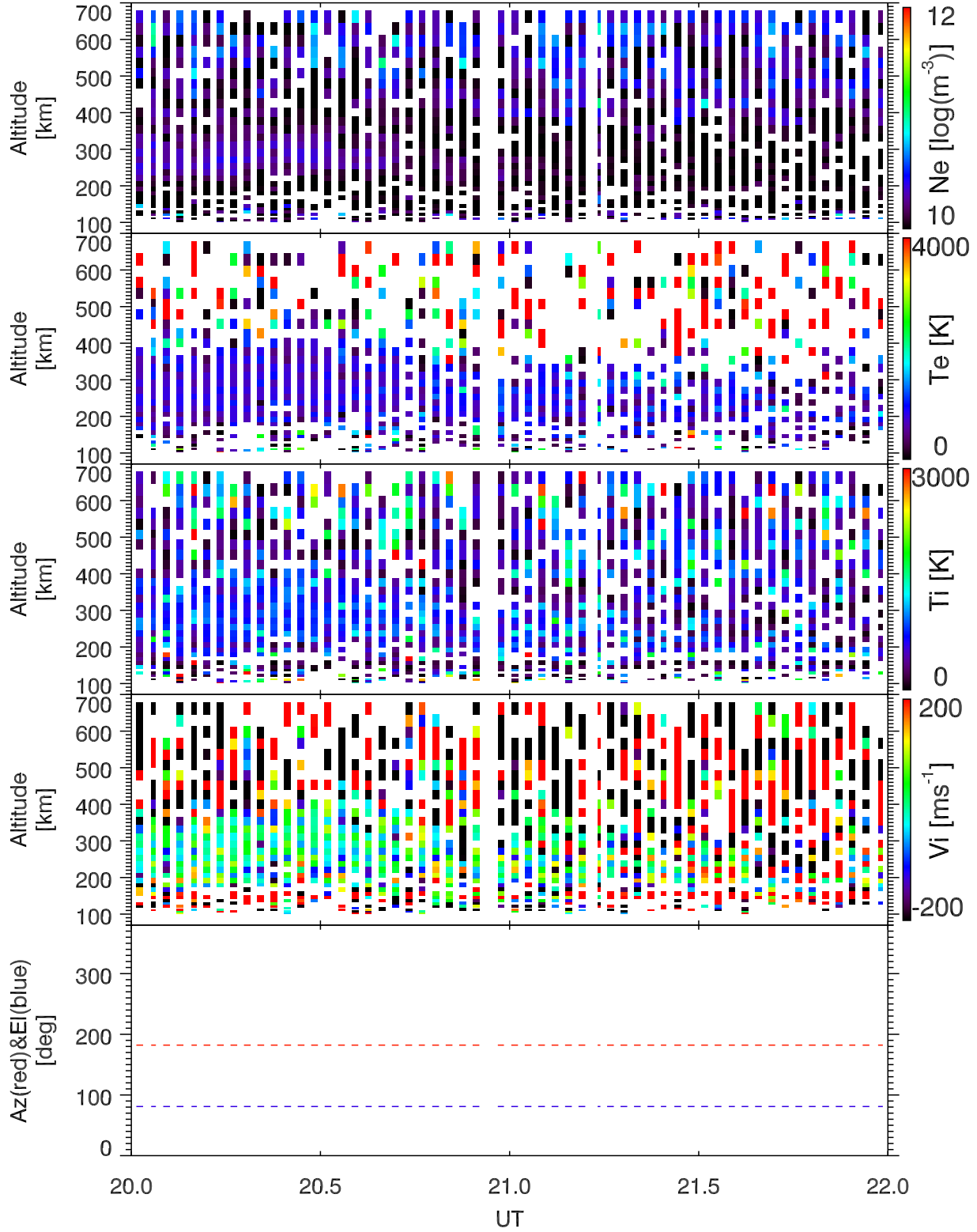
EISCAT 2005-11-09_20_22UT_tau0_ant@42m.
