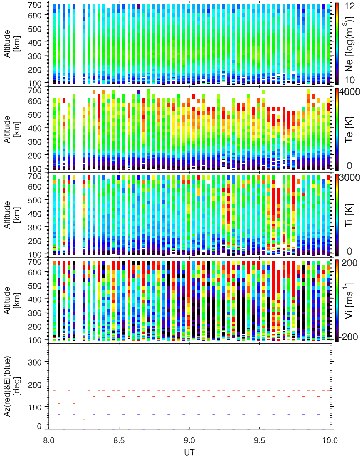
EISCAT 2003-03-23_08_10UT_tau0_ant@32m.
