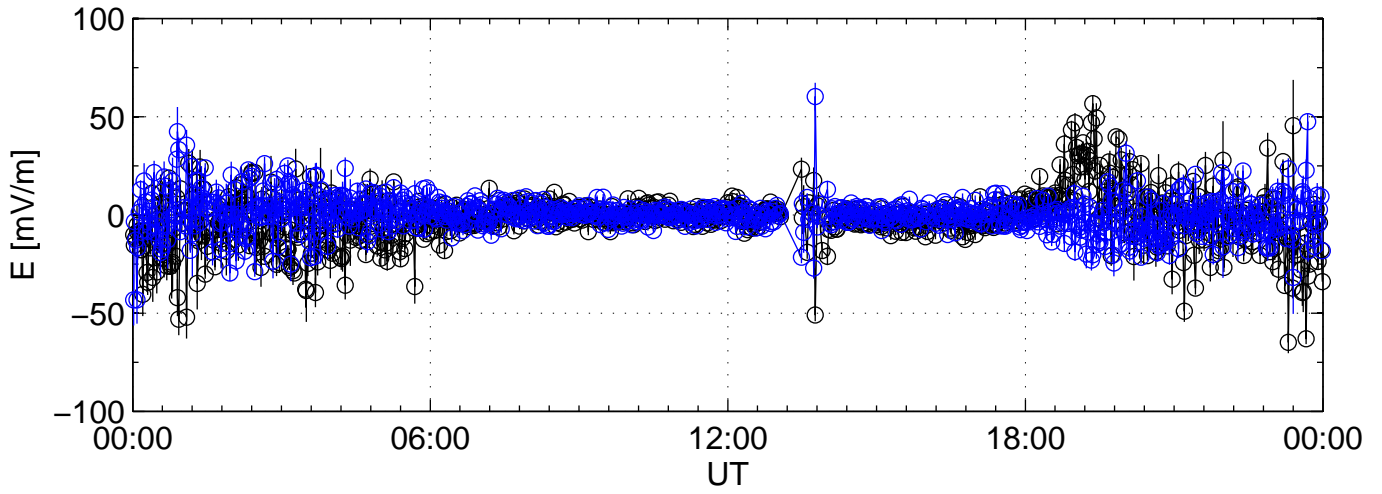
2005-09-23 kst t2pl 0000sec black:North, blue:East
