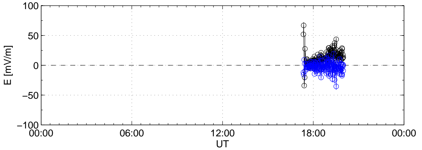
2002-09-27 kst cp1l 0060sec black:North, blue:East
